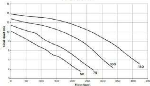
Flow Curves
