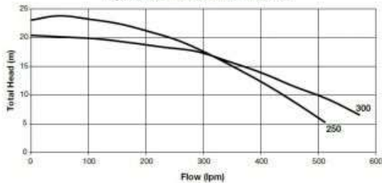
Hydrostorm Plus Flow Curves
