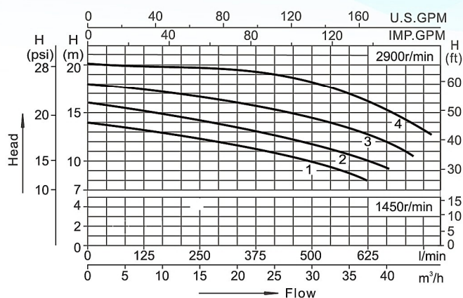
Performance curves
