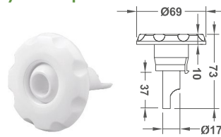
φ2-3/4" Face Eyeball Spa Jet
