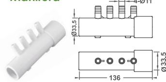
Port Air Manifold
