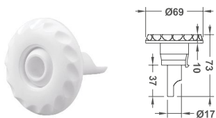
φ2-3/4" Vortex Face Eyeball Spa Jet
