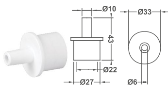
Barb Plug
