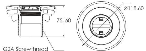
Vacuum Fitting (Vinyl Pool) EM2836
