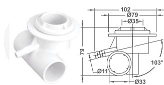
φ10mm Barb Air & φ25mm Water
