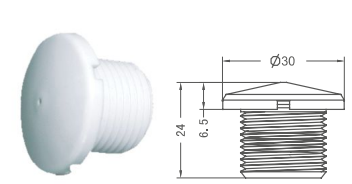
Single Hole Jet
