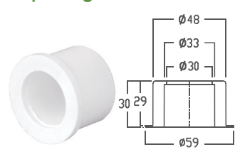
Pipe Plug
