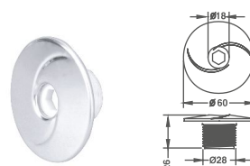
φ2" Face (Spiral) Jet
