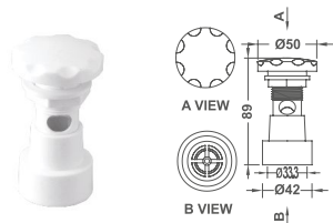
φ25mm Air Control
