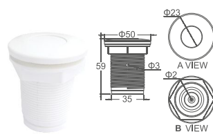
Air Button
