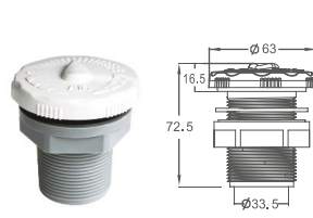
Standard Air Control
