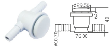
Twin Hole Air Jet
