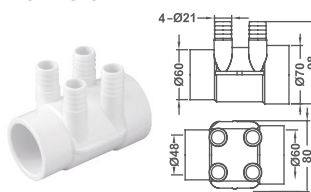
Port Water Barb Manifold
