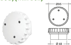
φ2 Section Drain Straight Body(with Bolt)
