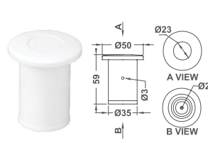
Air Button
