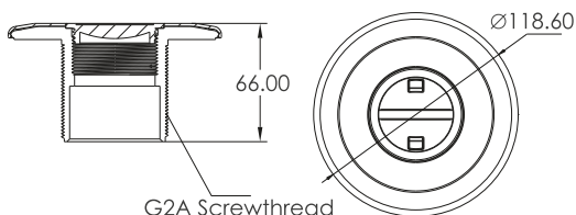
Vacuum Fitting (Concrete Pool) EM2831
