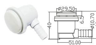
Single Hole Air Jet
