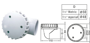
φ2 Section Drain Ell Body(Threaded)
