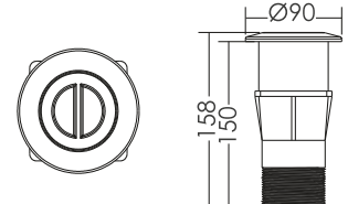
Vacuum Fitting (Concrete Pool)
