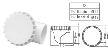
φ2 Section Drain Ell Body(Slip Fit)
